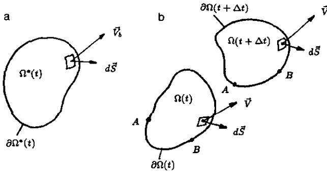
FIG. 1. Definition of a control volume and material volume. (a) Control volume, denoted by “*”, may be nonstationary, e.g., on rotating frame. (b) Material volume, \vec{V}_b = \vec{V} .
