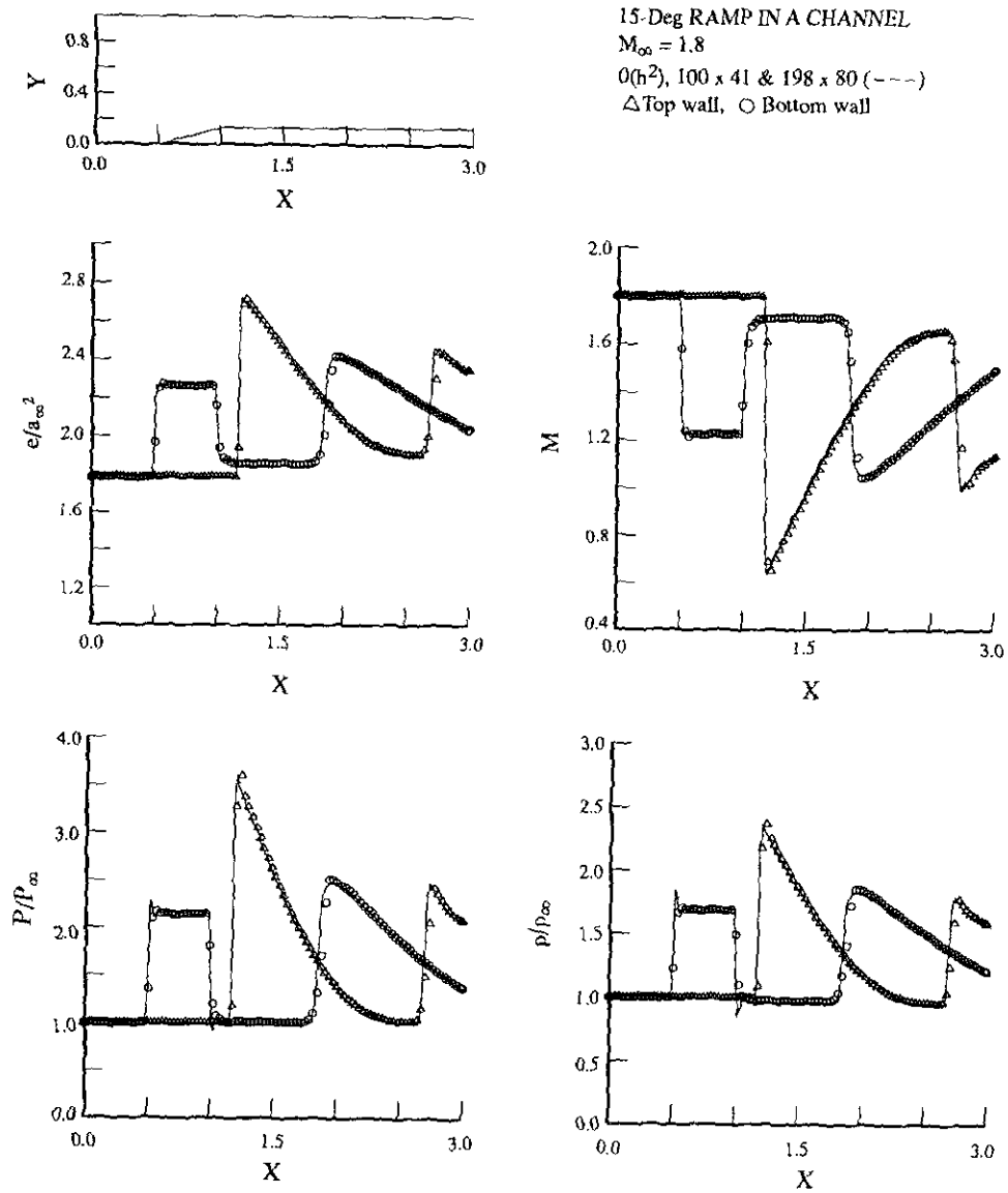
FIG. 12. Distributions of variables on top and bottom walls for M_{\infty} = 1.8 , 15^\circ ramp flow; lines are Eulerian solution ( 198 \times 80 grid) and symbols are Lagrangian solution ( 100 \times 41 grid) with \Delta and \circ denoting top and bottom walls, respectively.
