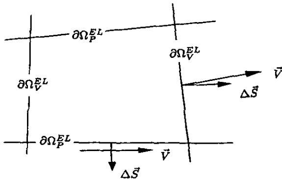
FIG. 2. Definition of an Extended Lagrangian volume: the cell boundary \partial\Omega^E_P is parallel to the fluid velocity \vec{V} .
